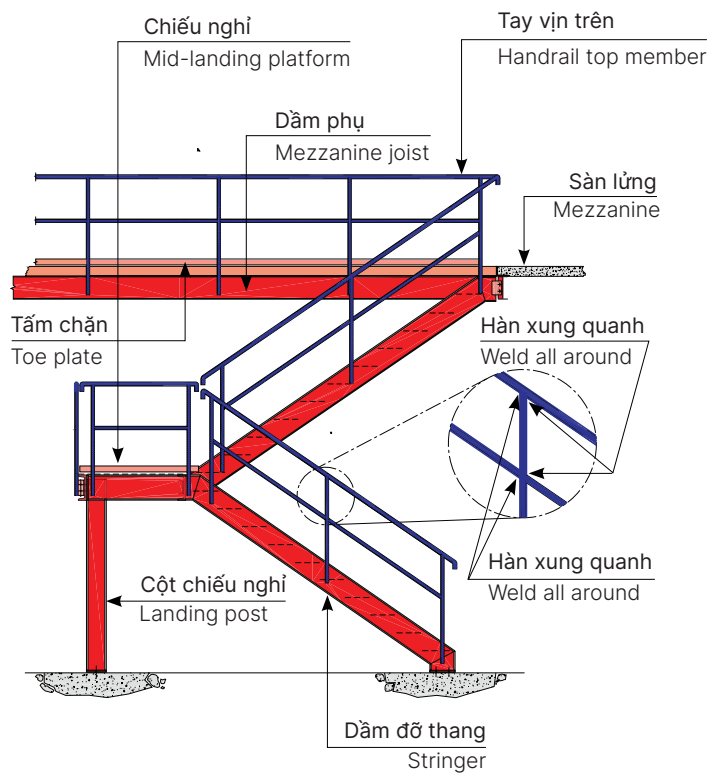
LAN CAN HANDRAIL
