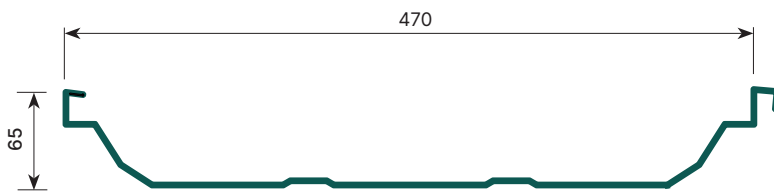
TÔN SÓNG SEAMLOCK | LOCKSEAM PANEL
