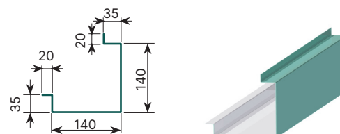
DIỀM ỐP GÓC | OUTSIDE CORNER TRIM
